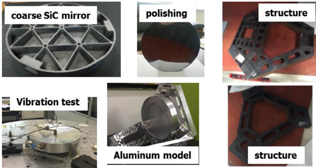
Fig. 5. The development of telescope (up left is the coarse SiC primary mirror, up middle is the polished SiC primary mirror, up right and down right is the SiC telescope structure, down middle is the aluminum telescope model, down left is the vibration test of the aluminum model).
